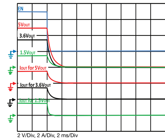
Fig. 23 - Typical Fall Time C_{OUT} = 200 \mu F, C_{IN} = 4.7 \mu F, I_{OUT} = 1.5 A
