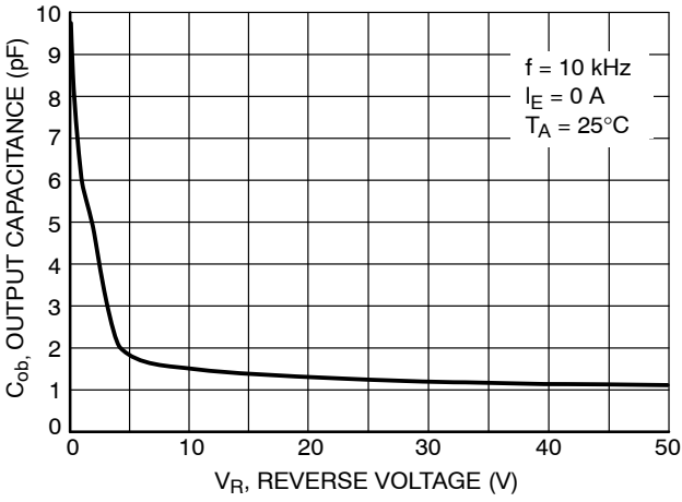
Figure 117. Output Capacitance
