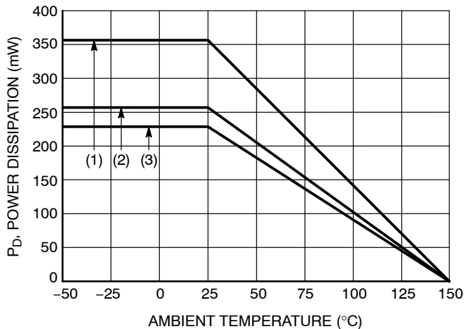
Figure 109. Derating Curve
