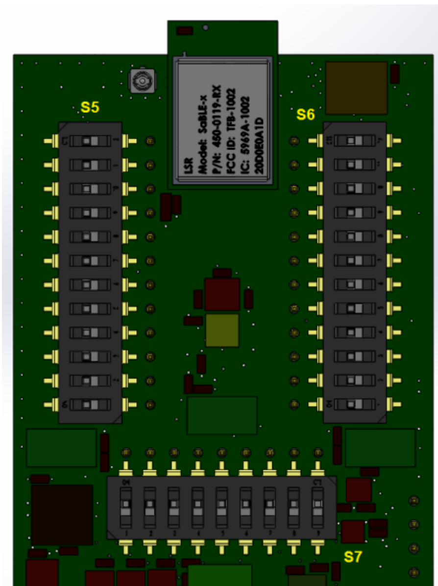
Figure 6 Bus Isolation Switches
