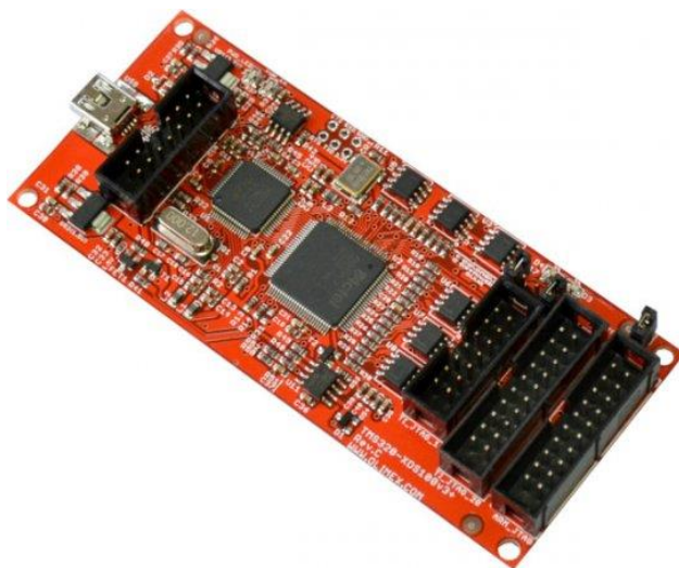
Figure 16 Olimex TMS320-XDS100-V3 JTAG Debugger/Programmer
